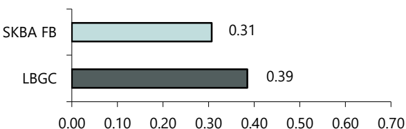
Convexity
