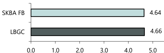
Effective Duration
